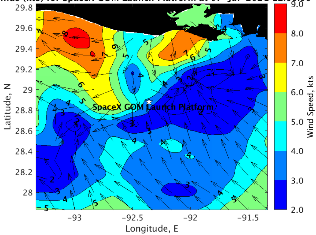
Winds (kts) for SpaceX GOM Launch Platform at 07-Jul-2021 12:00:00
